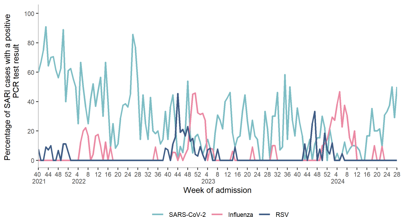
Figure 3: Percentage of SARI cases with a positive laboratory test result for SARS-CoV-2, influenza and RSV by week, from week 40 2021 to week 28 2024.
