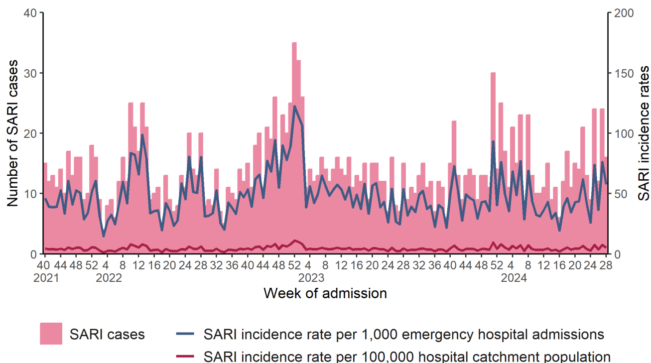
Figure 1: Number and incidence of SARI hospitalised cases (emergency admissions) by week of hospital admission, week 40 2021 to week 28 2024 (n=1414)
